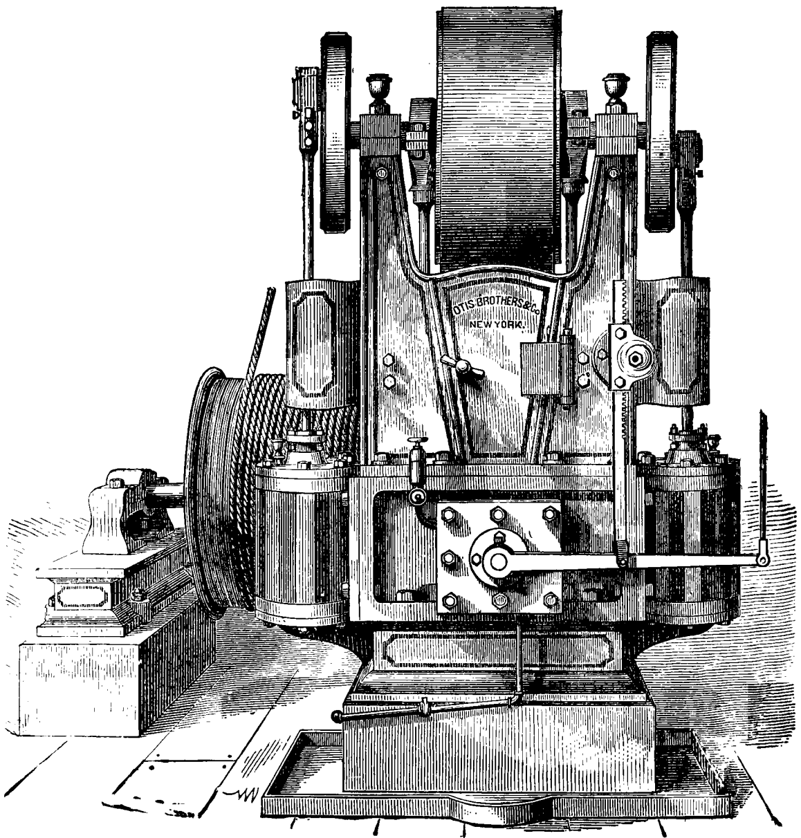
FRONT VIEW OF THE OTIS ENGINE AND WINDING DRUM.
